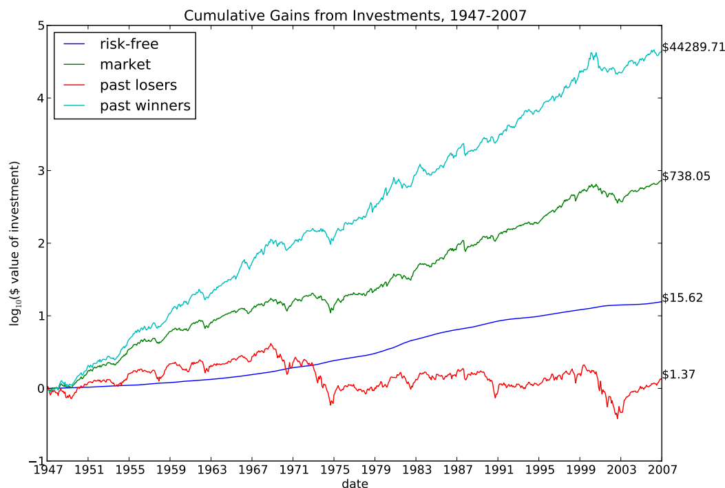
Figure 2: Momentum Components, 1947-2007
